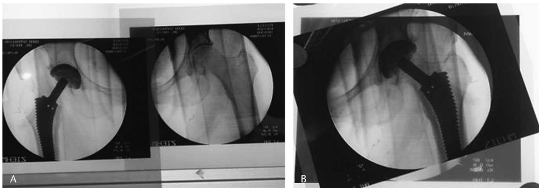
Fig 9A–B. The image intensifier is used to obtain an image of the unaffected hip. An image is taken of the trial components in the reduced position, and the two images are superimposed. The radiographic landmarks of the pelvis are lined up and the landmarks of the femur are compared to verify correct length and offset.
